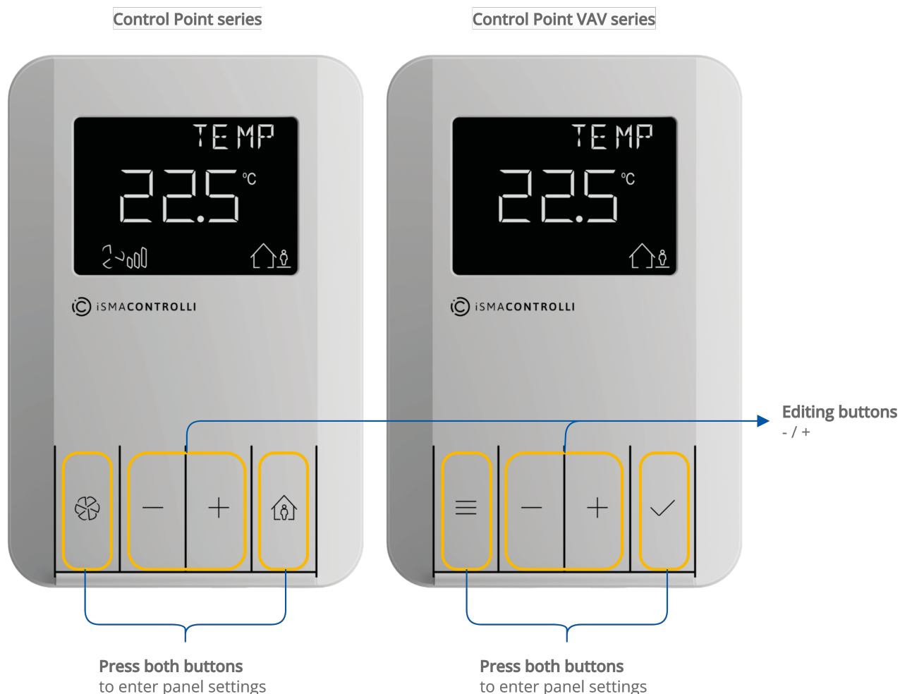
Figure 23. Editing settings
